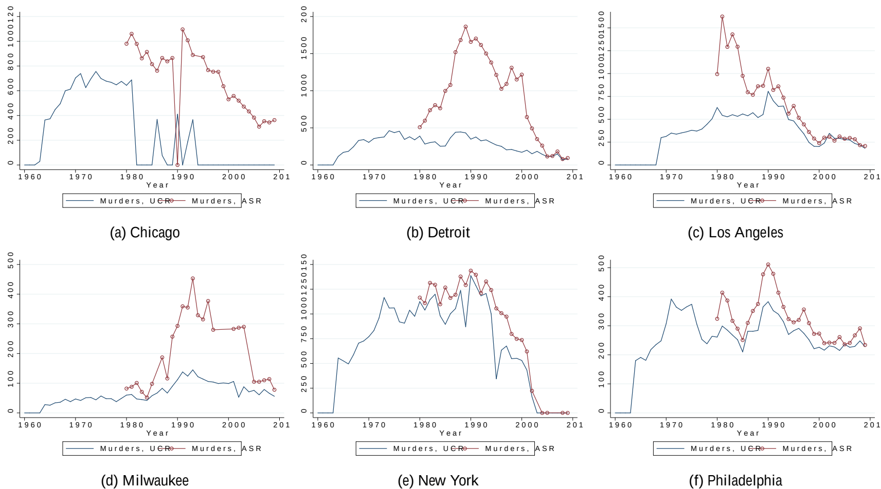
Figure A.4: The Relationship Between the Number of Murders Cleared by Arrest in UCR and ASR Data, 1960-2009, Severe Measurement Error Cities
