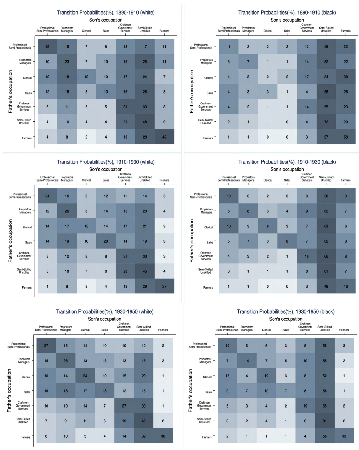
Figure A.9: Transition Probabilities by Occupation Groups: 7 Categories
