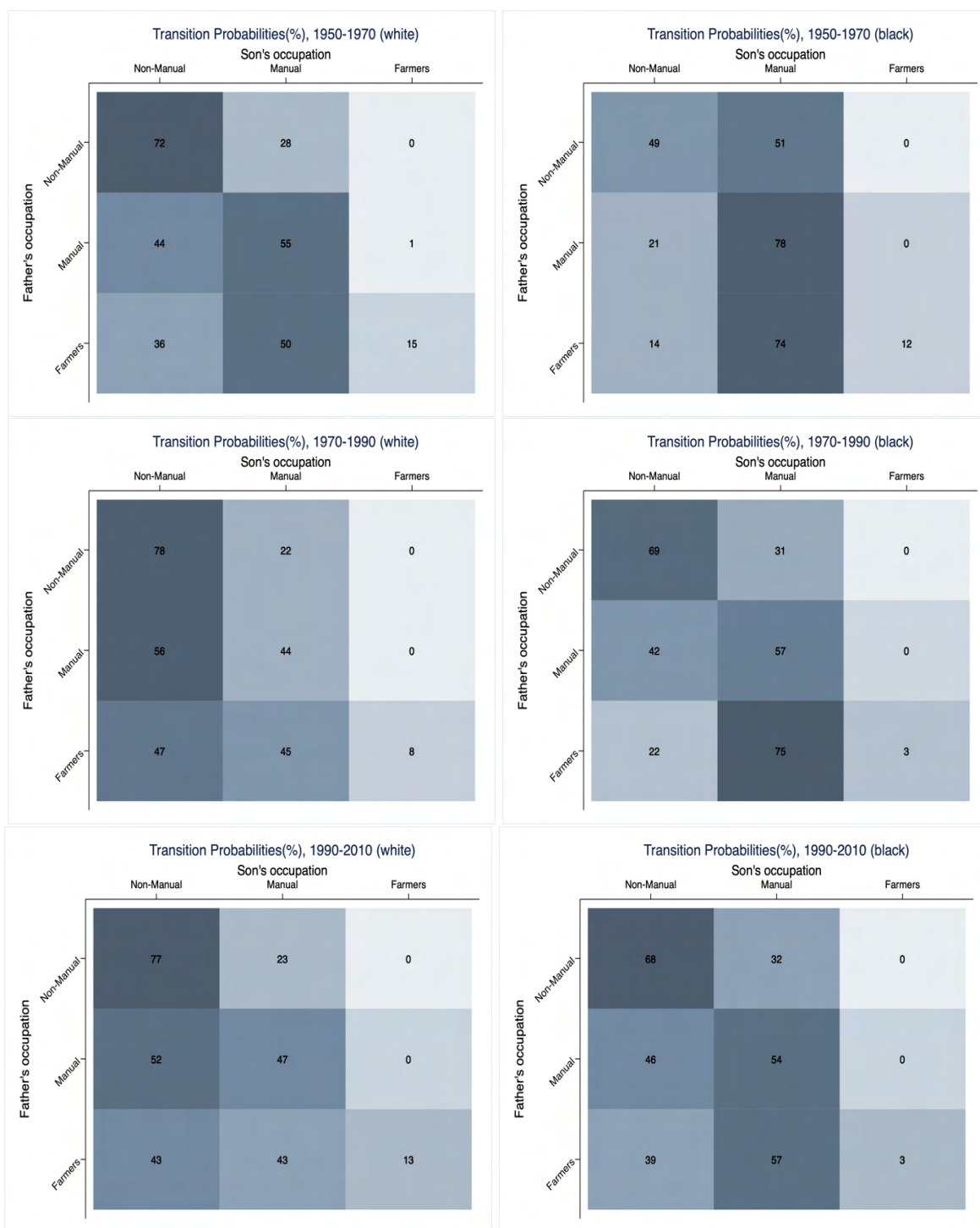
Figure A.6: Transition Probabilities by Occupation Groups: 3 Categories
