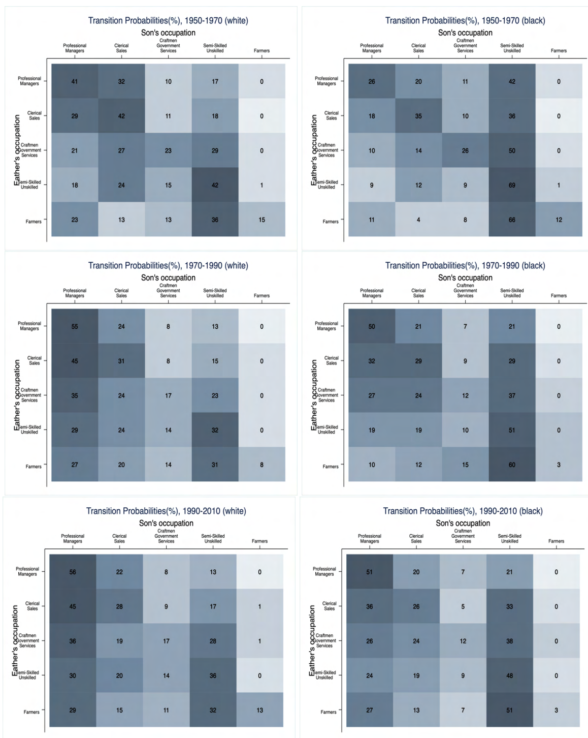
Figure A.8: Transition Probabilities by Occupation Groups: 5 Categories
