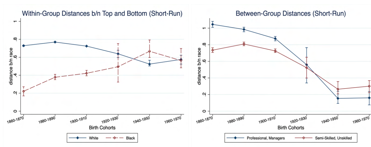
Figure 10: Within and Between Group Convergences (Short-Run)
