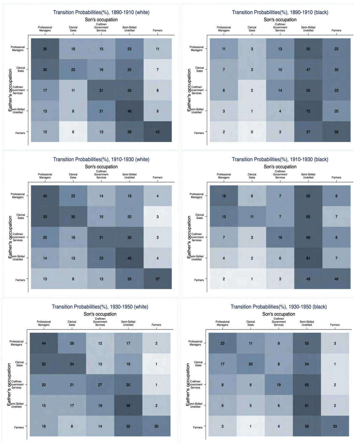
Figure A.7: Transition Probabilities by Occupation Groups: 5 Categories
