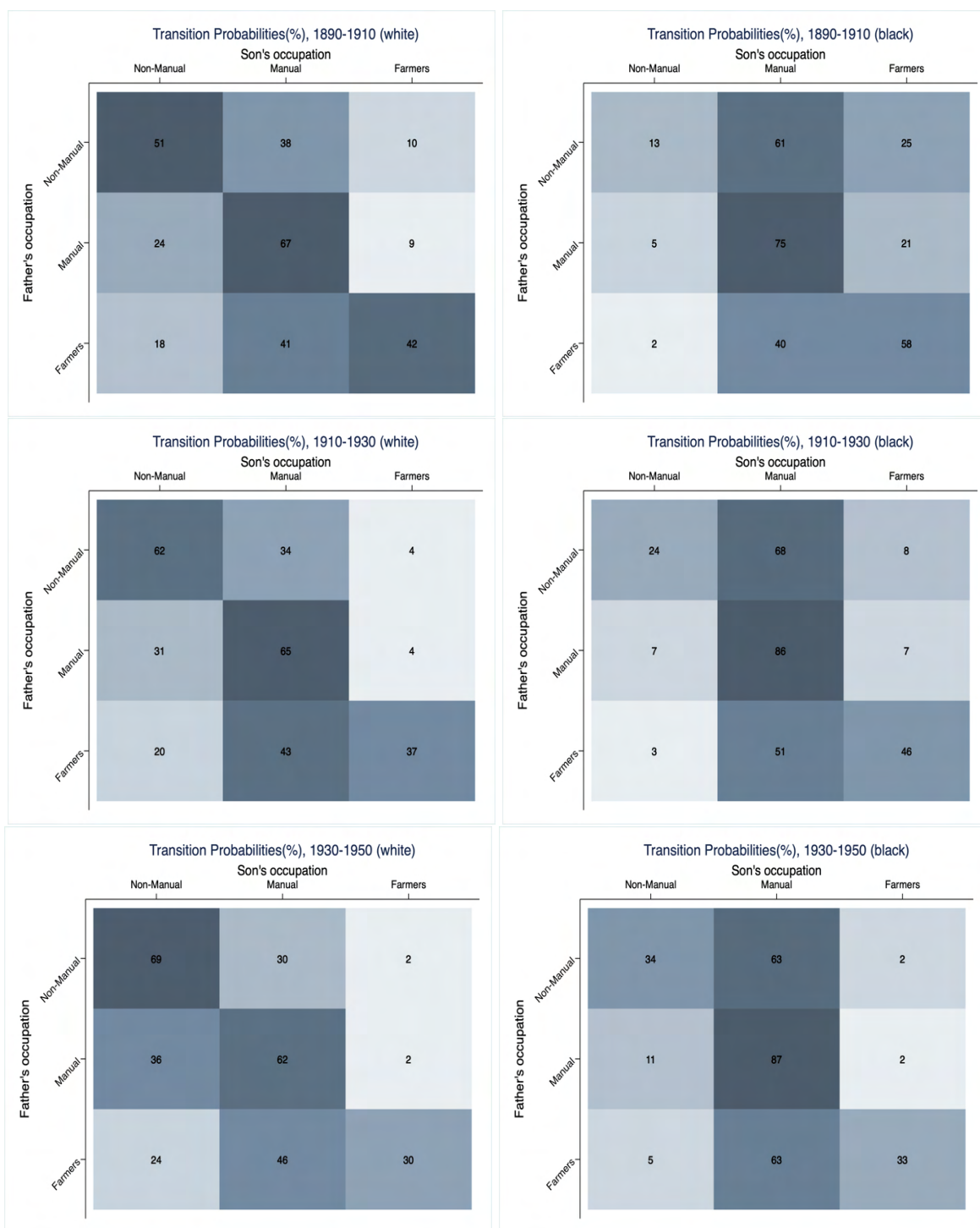
Figure A.5: Transition Probabilities by Occupation Groups: 3 Categories
